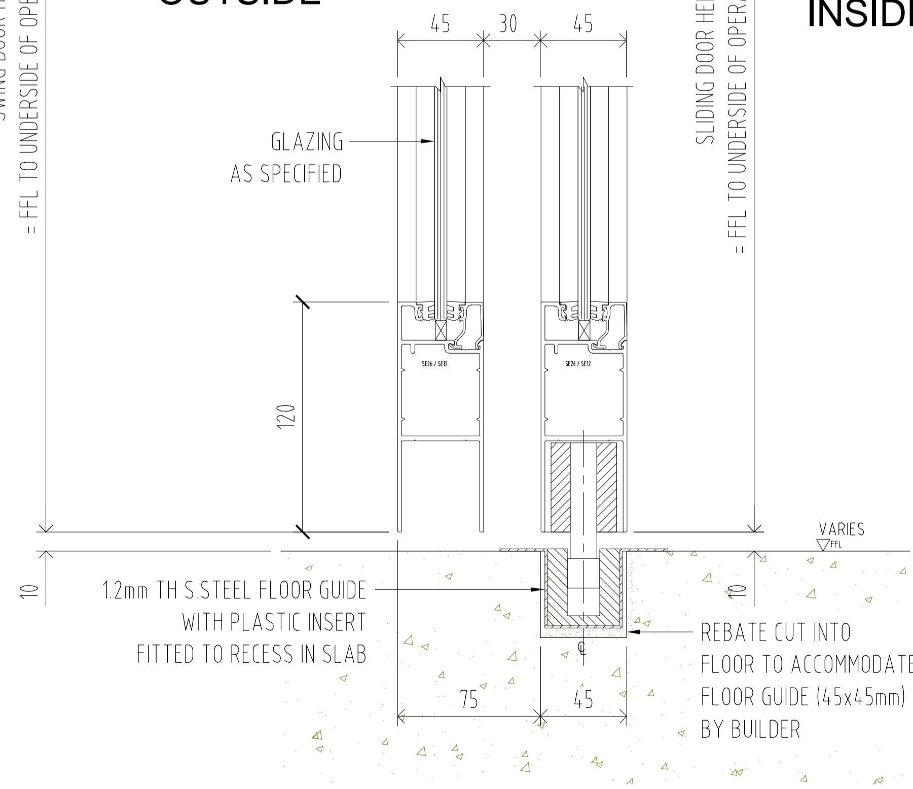
A 009 VERTICAL DETAIL SCALE: 1:2
