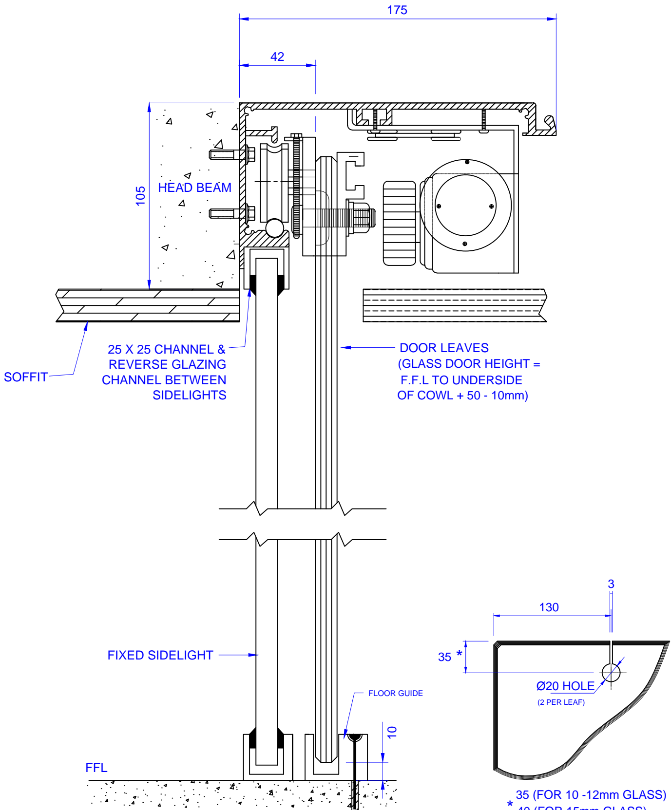
GLASS DRILLING DETAIL
