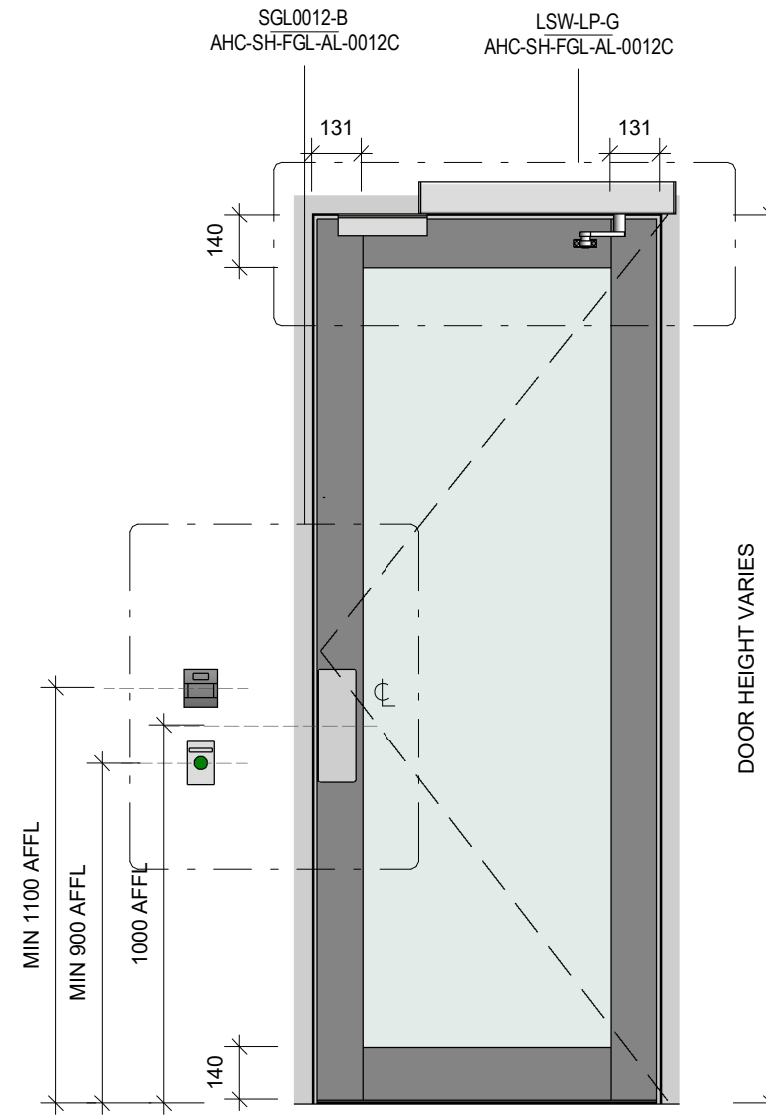
INSIDE ELEVATION PUSH SIDE
