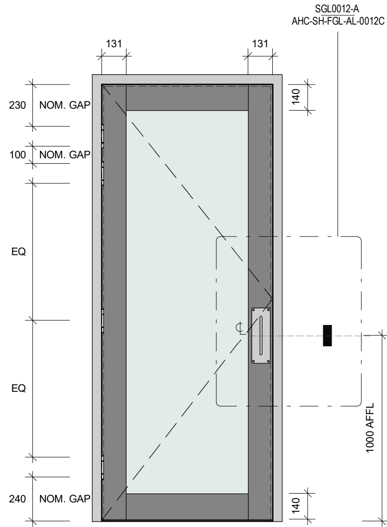
OUTSIDE ELEVATION PULL SIDE
