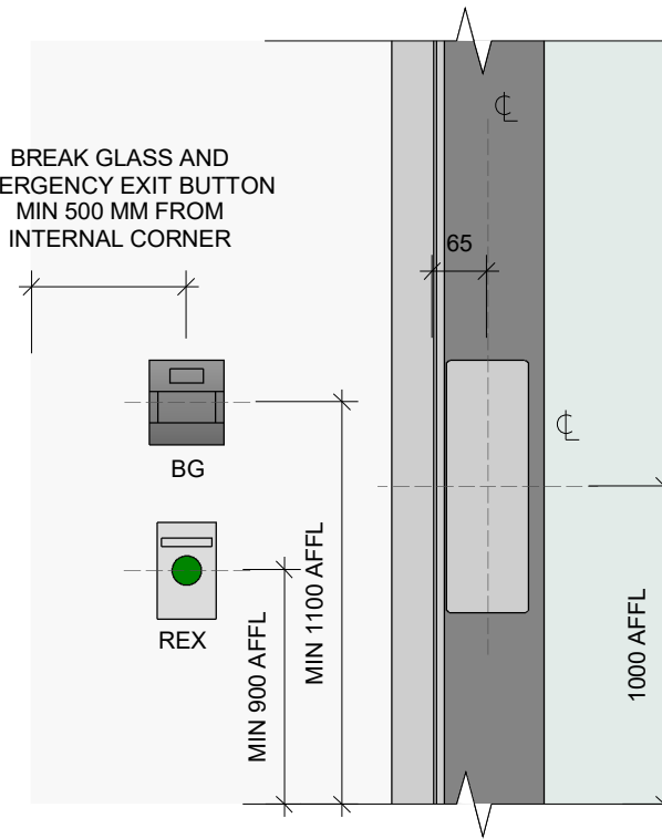
SGL0012-B PUSH SIDE
